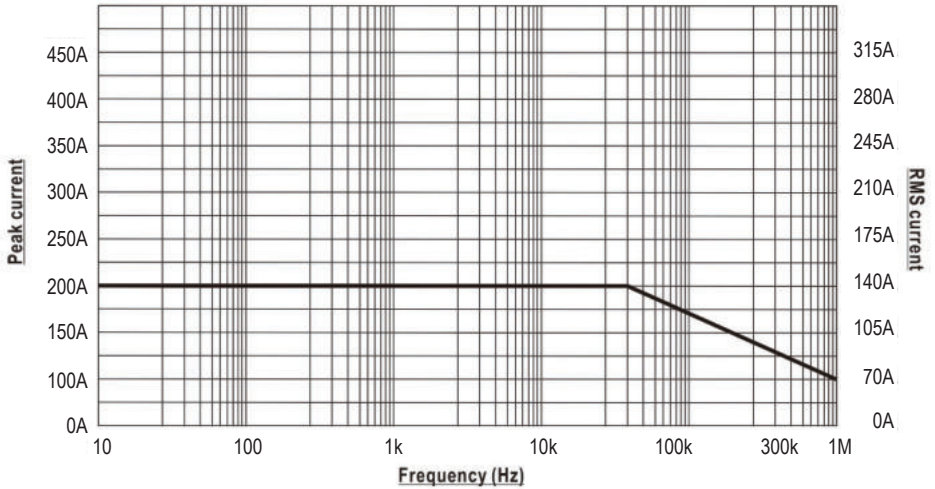
Figure 7: Maximum current versus frequency
