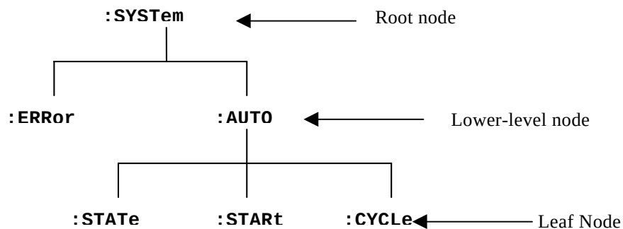
Figure 4: Tree hierarchy
