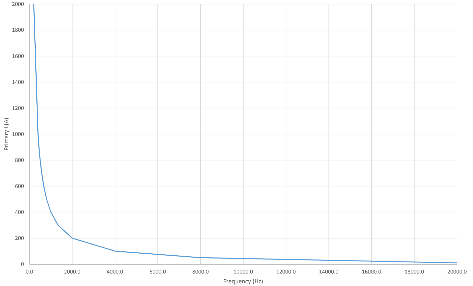
TA167 Frequency derating curve
