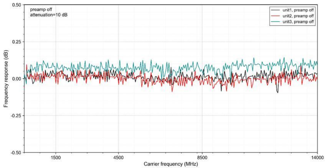
Measured frequency response of RSA804/RSA808/RSA814
