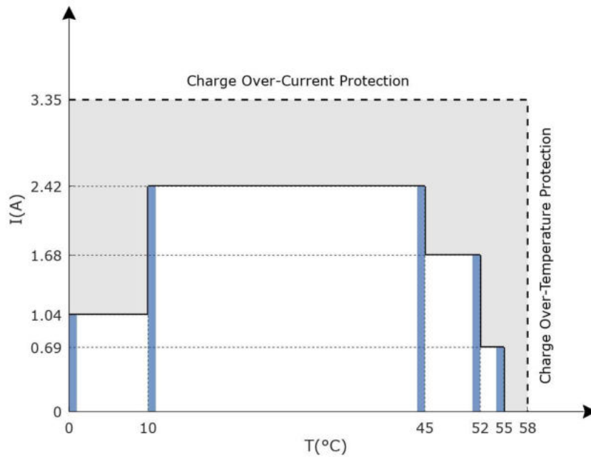
JEITA profile for Panasonic type
