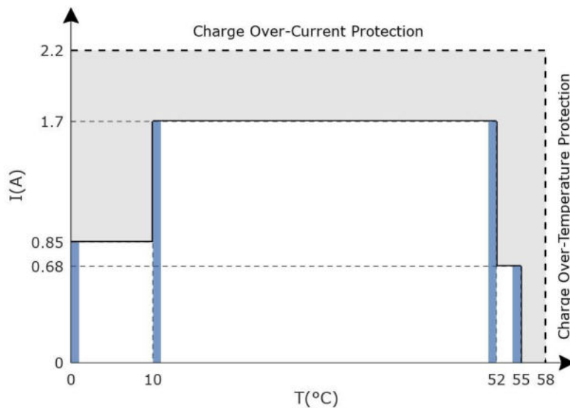
JEITA profile for Samsung type
