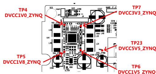
Figure 41 Test points for the processor power supplies
