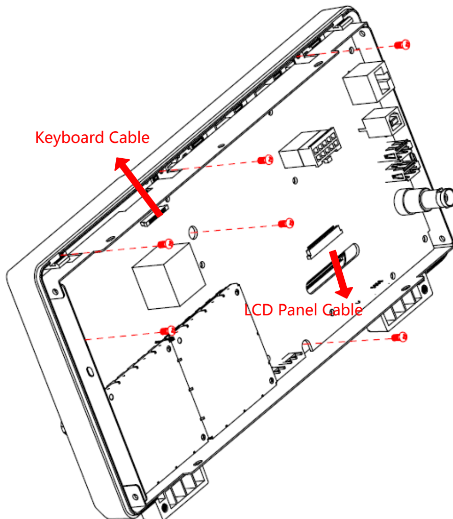
Figure 28 Removing the front cover
