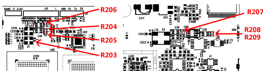
Figure 42 Test points for clock
