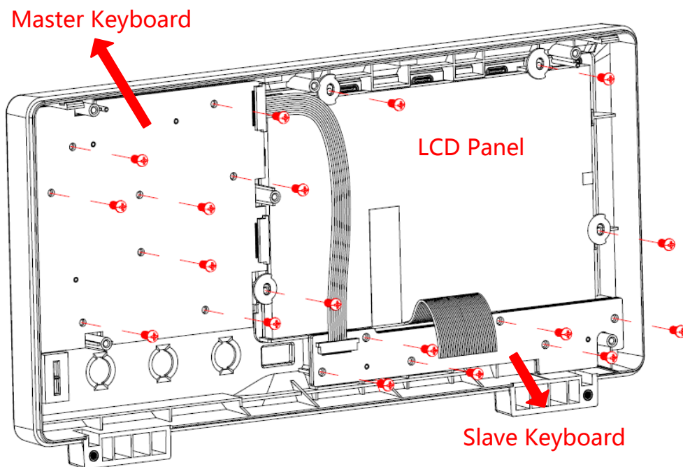
Figure 23 Removing the LCD panel and keyboard
