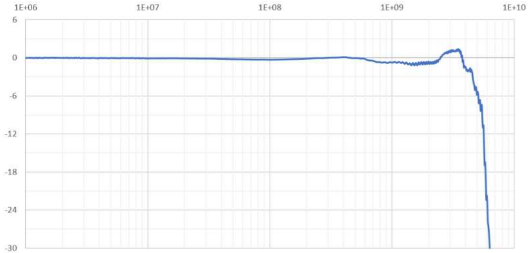
SRP-45 frequency response curve
