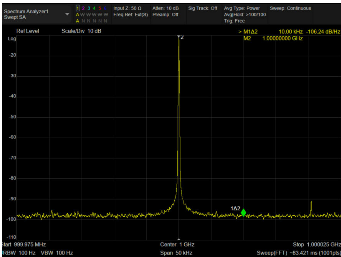
Figure 2-1 Typical Phase Noise Measurement Methods
