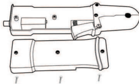
Figure 5: Battery Change
