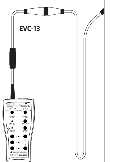
Charging Station Type 1 (with fixed cable)
