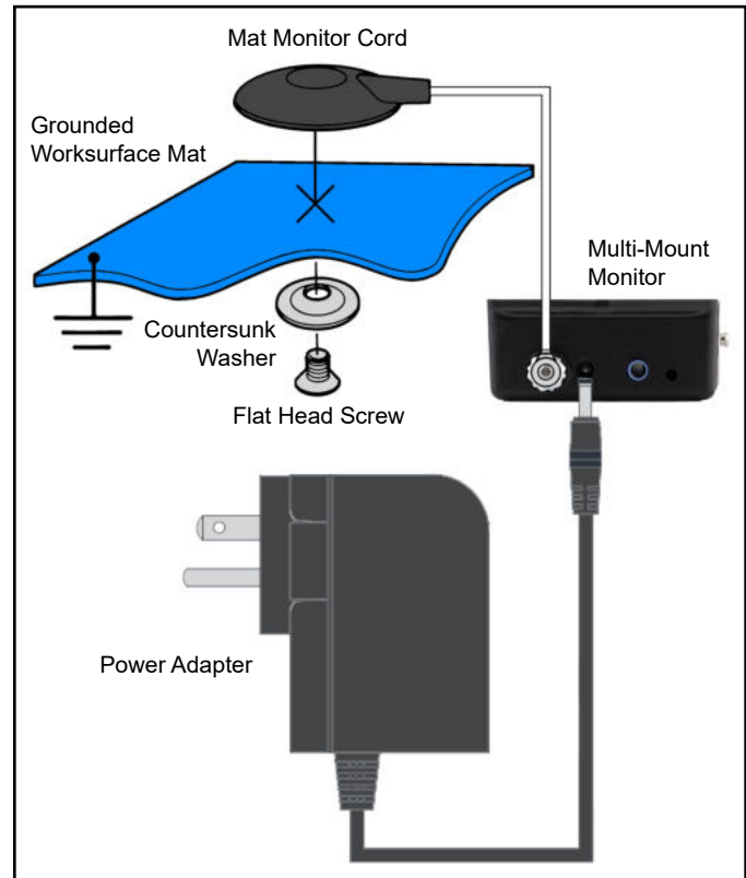
Figure 4. Installing the Multi-Mount Continuous Monitor
