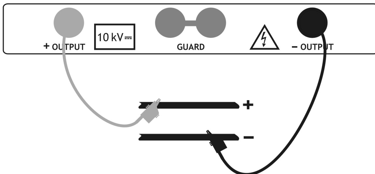
Fig. 15: Connection of meter for voltage measurement
