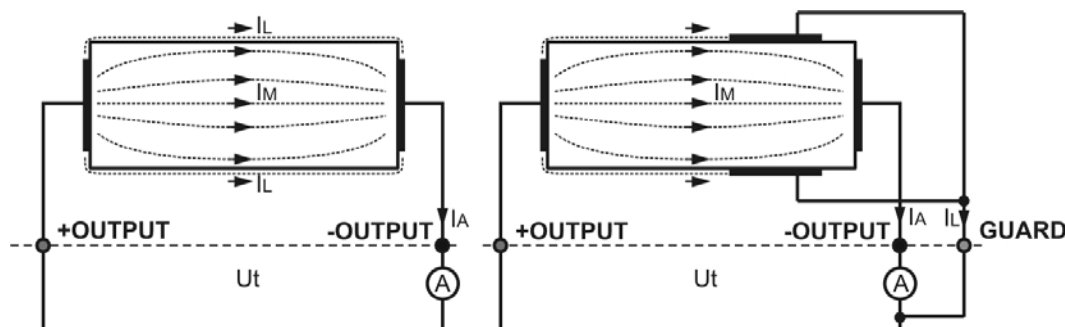
Fig. 11: Principle scheme relative to the Guard terminal
