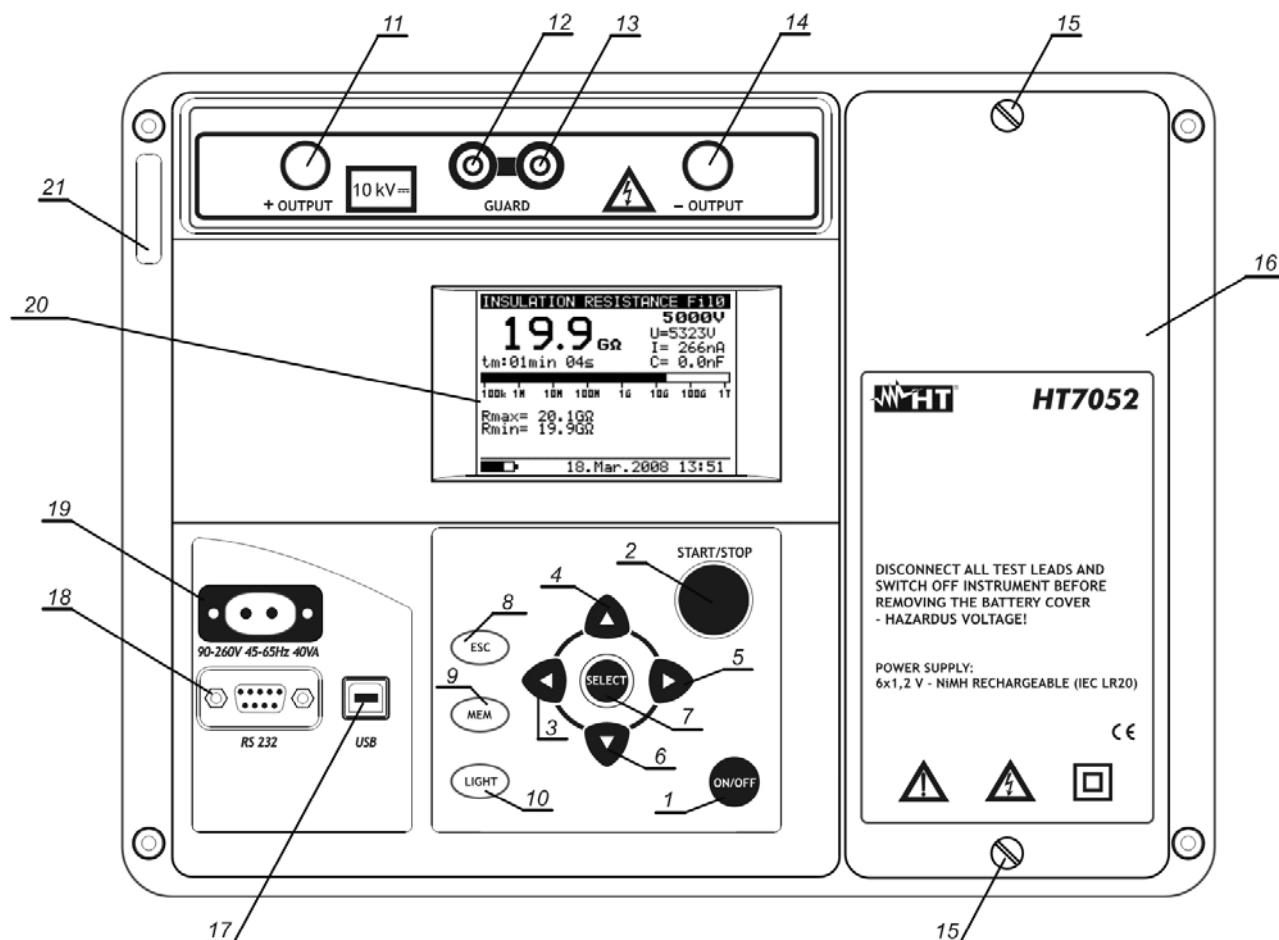
Fig. 1: Instrument description
