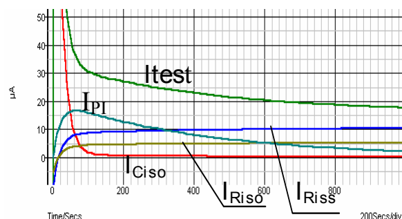
Fig. 8: Current graphs
