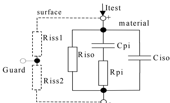
Fig. 7: Equivalent electrical circuit
