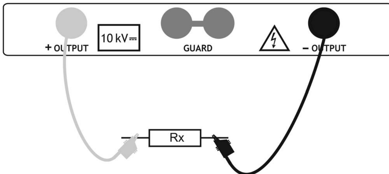
Fig. 46: Connection of instrument for withstanding test
