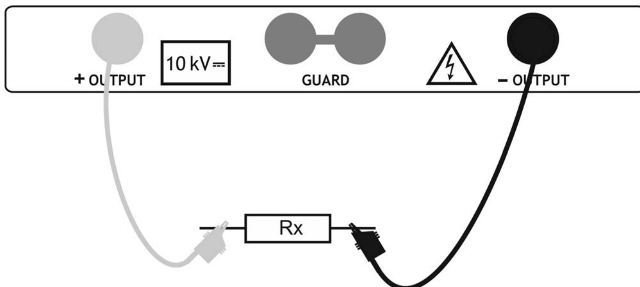
Fig. 42: Connection of instrument for insulation measurement
