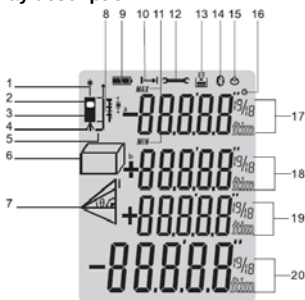
Fig. 2: Description of the symbols at display
