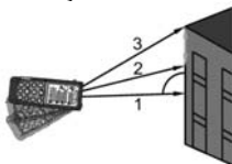
Fig. 11: Indirect 3-point measurement – Mode 2
