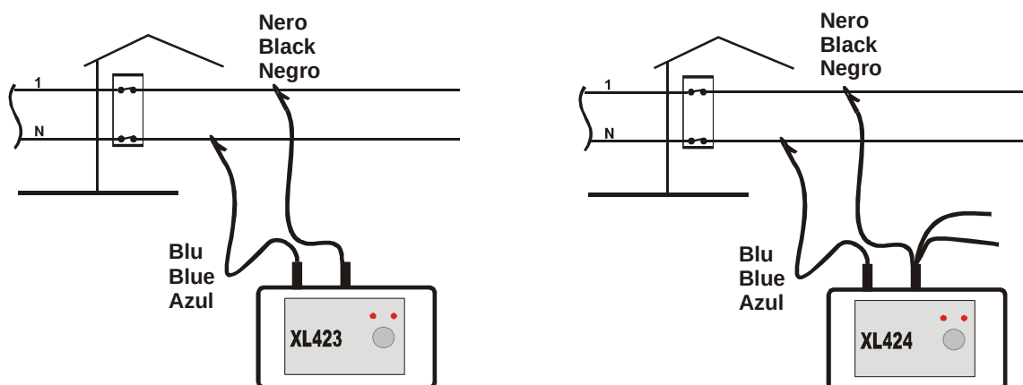
Fig. 2: Instrument's connection in Single Phase plant
