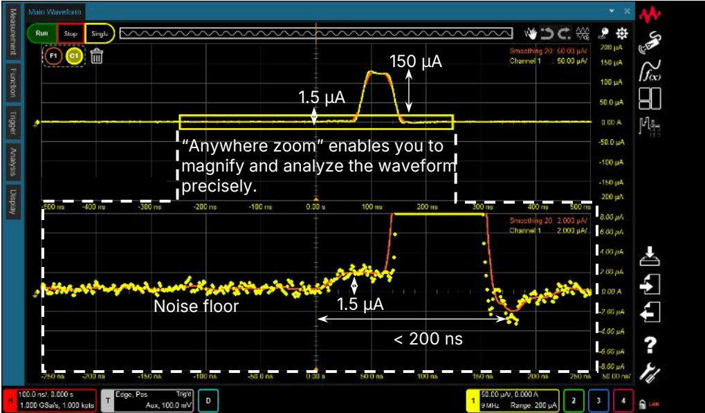
Figure 6. Low current behavior can be unveiled by sensing technology and Anywhere Zoom.
