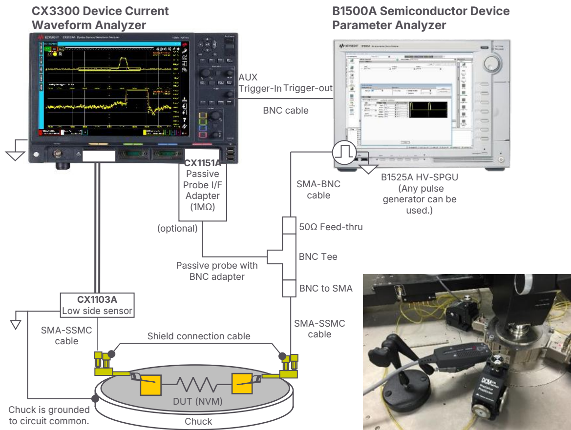
Figure 7. On-wafer measurement setup example
