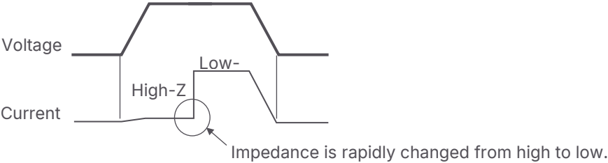
Figure 5. Dynamic current changes in a pulse
