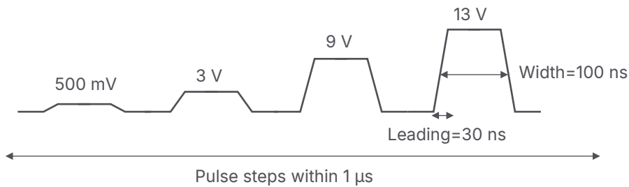
Figure 3. Sample narrow step pulses
