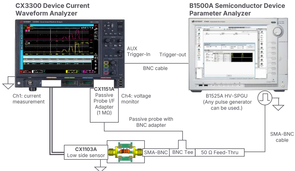
Figure 2. Setup example using a discrete device
