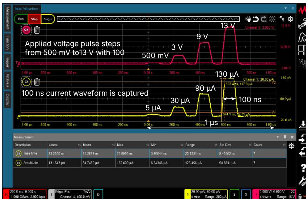
Figure 4. 100 ns current waveform is visualized
