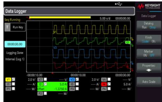
Figure 9. Data logger mode
