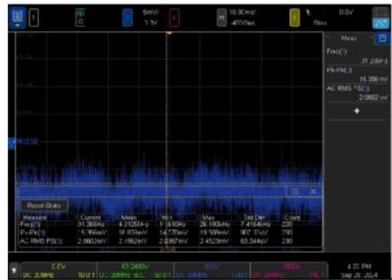
Figure 4. E36441A delivers clean power with low output noise (10x amplification as shown)
