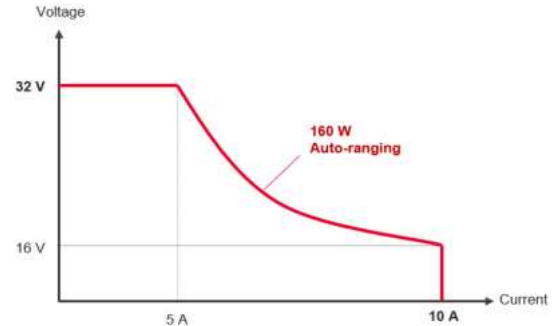
Figure 1: Autoranging technology
