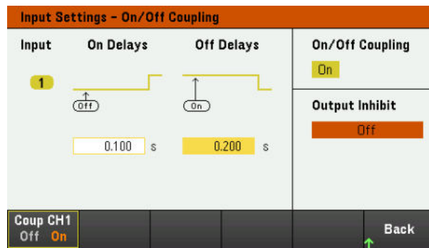
Load mode
