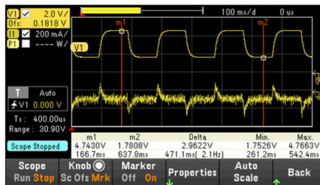
Figure 10. Scope View.
