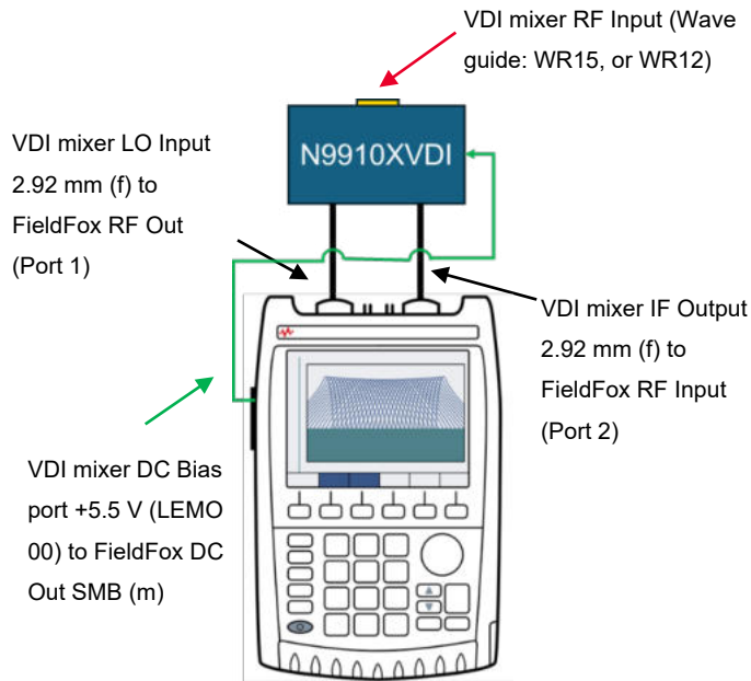
Figure 1. VDI PSAX frequency extender diagram
